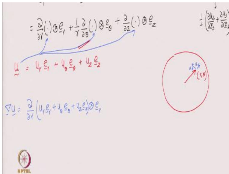
Figure 1: A typical section of an arbitrary body parallel to z plane: a point with coordinates (r, \theta) with respect to the origin of cylindrical coordinate system is also shown along with the components of displacement along basis directions.
